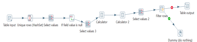
Fig. 2. Cleaning transformation in cleaning_sales.ktr .
